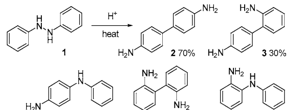
Scheme 1. Benzidine Rearrangement of Hydrazobenzene 1
